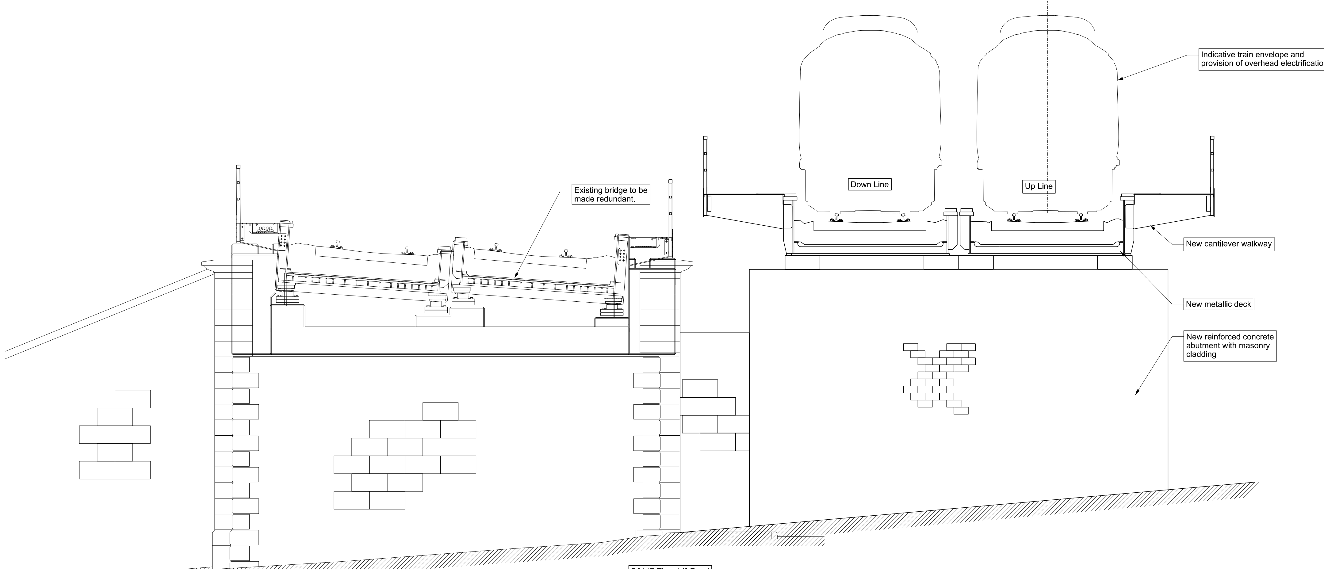
Section CC Proposed: Thornhill Road Underbridge (MDL1/9) Scale 1:50
