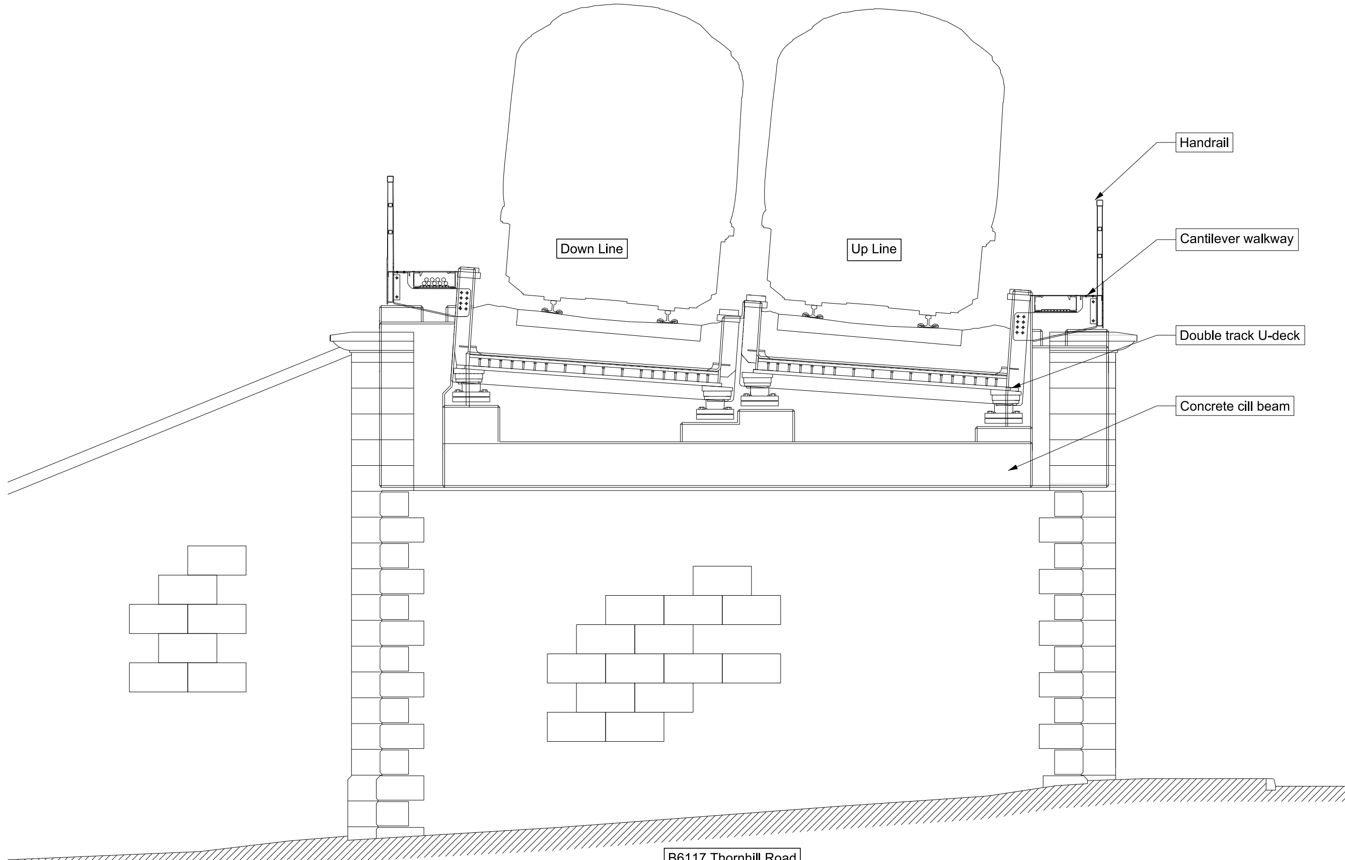
Section CC Existing: Thornhill Road Underbridge (MDL1/9) Scale 1:50
