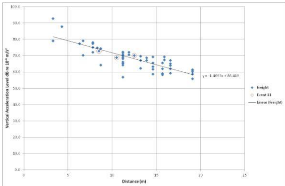
Figure 49. Freight train decay characteristics at 160Hz
