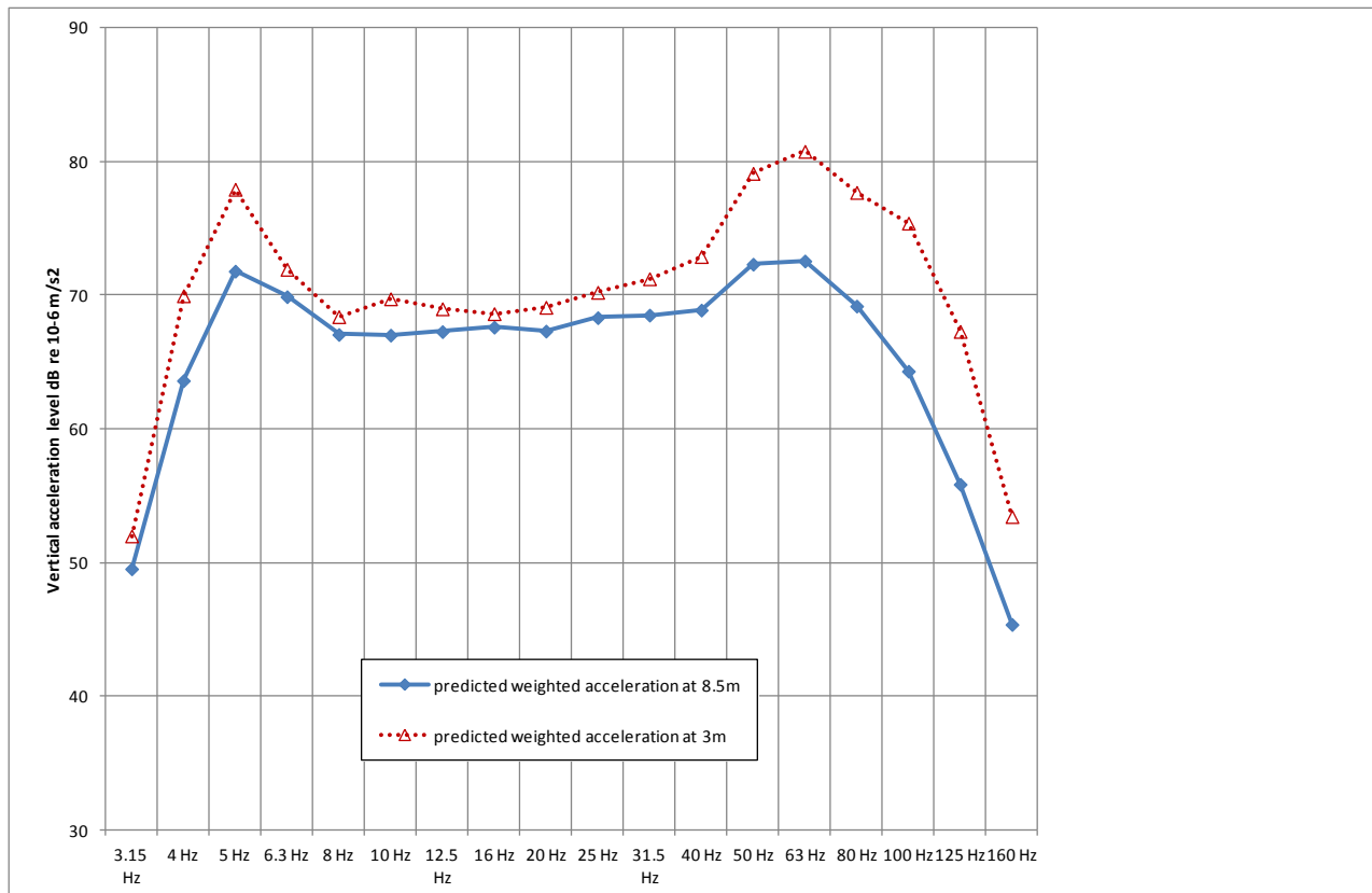
Figure 23. Predictions undertaken using the decay curves through event 11 data
