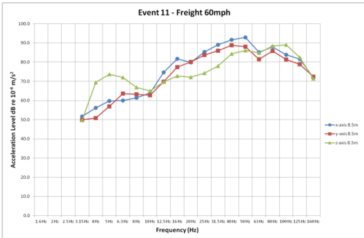
Figure 10. Acceleration 1/3 Octave Frequency Data – Stone Freight (X, Y & Z - Axis)
