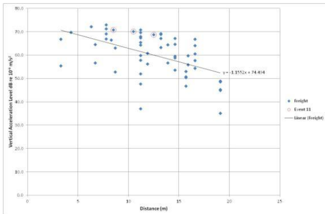
Figure 34. Freight train decay characteristics at 5Hz
