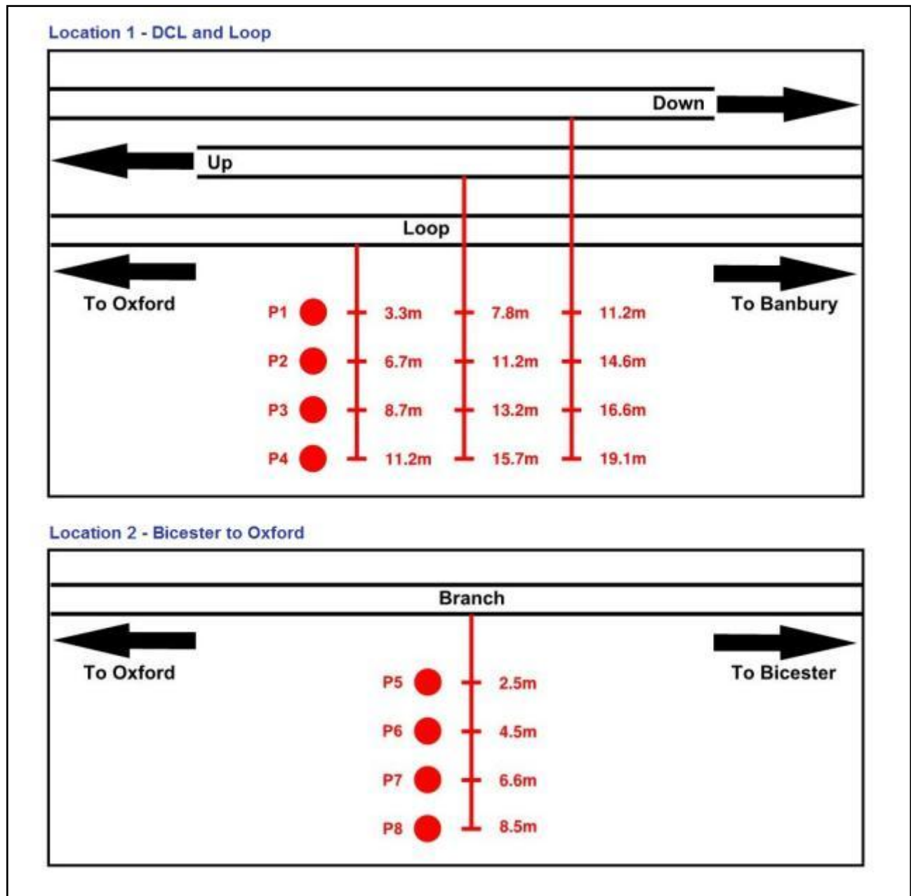
Figure 5. Measurement Positions in Relation to Track (October)
