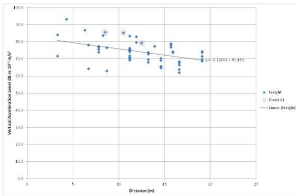
Figure 44. Freight train decay characteristics at 50Hz
