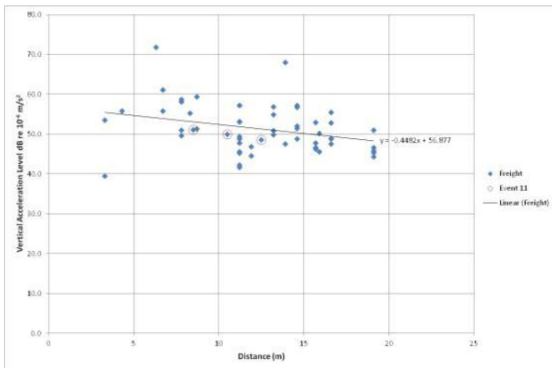
Figure 32. Freight train decay characteristics at 3.15Hz
