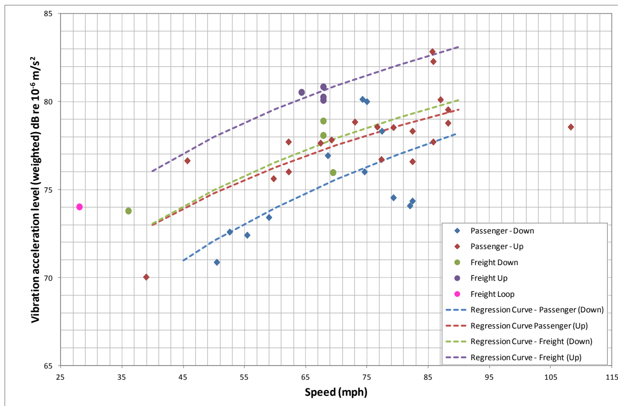
Figure 13. Measurements at Control Position
