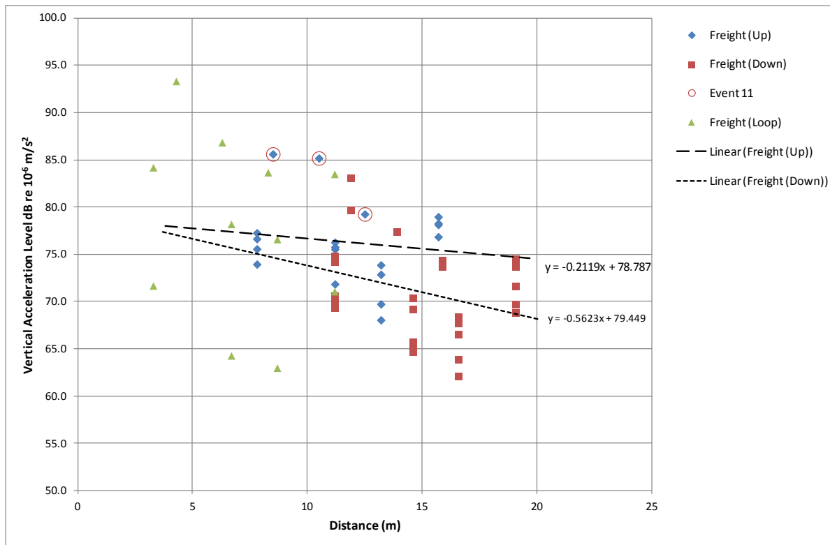
Figure 17. Freight train, influence of track at 63Hz
