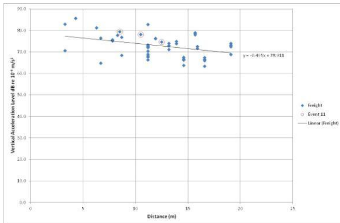
Figure 42. Freight train decay characteristics at 31.5Hz
