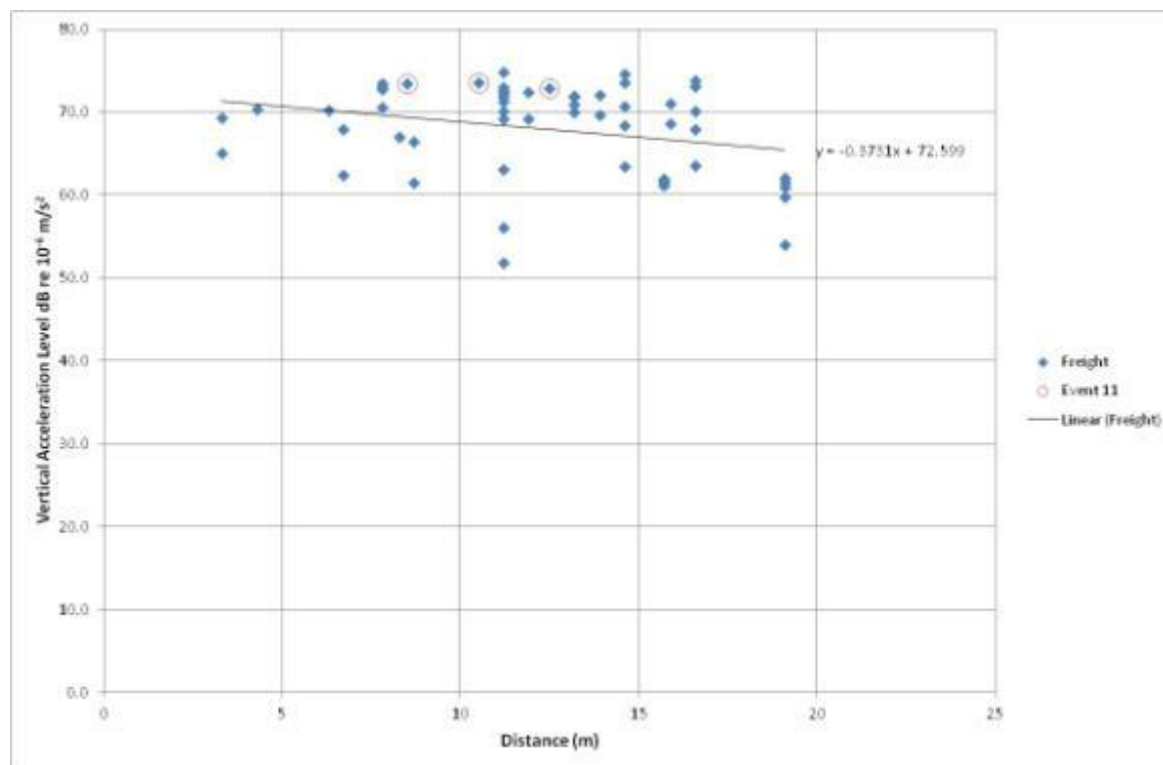
Figure 36. Freight train decay characteristics at 8Hz
