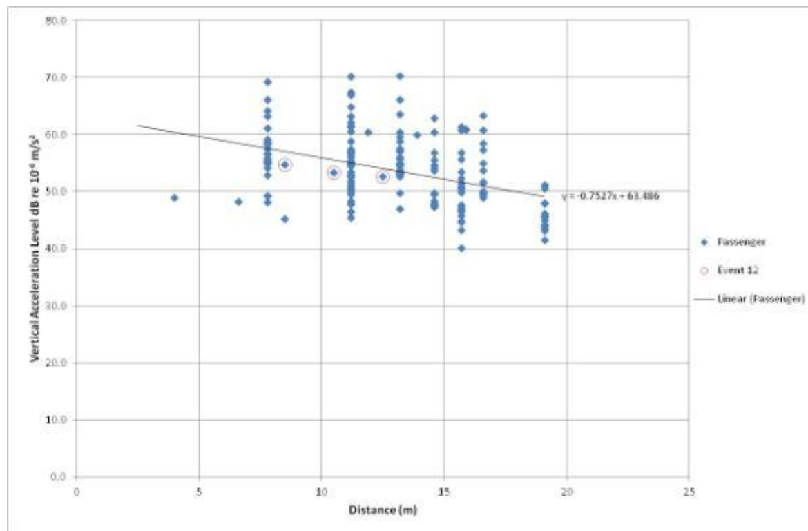
Figure 51. Passenger train decay characteristics at 8Hz
